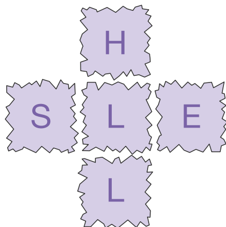
Figure 13.1 SHELL model.
